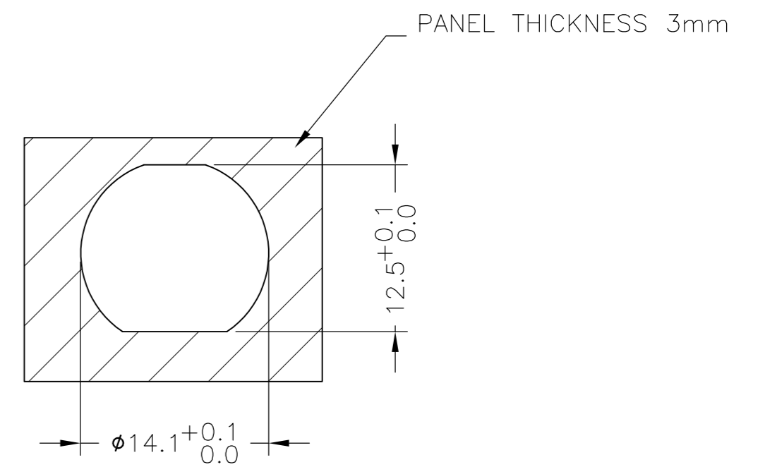
PANEL CUTOUT
